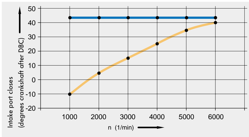
— Rigid camshaft — Variable camshaft
