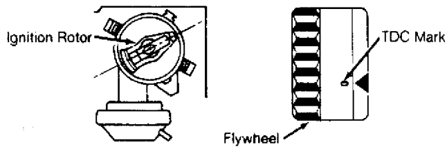
Fig. 7: Aligning Ignition Rotor (1.8L) Courtesy of Volkswagen United States, Inc.
